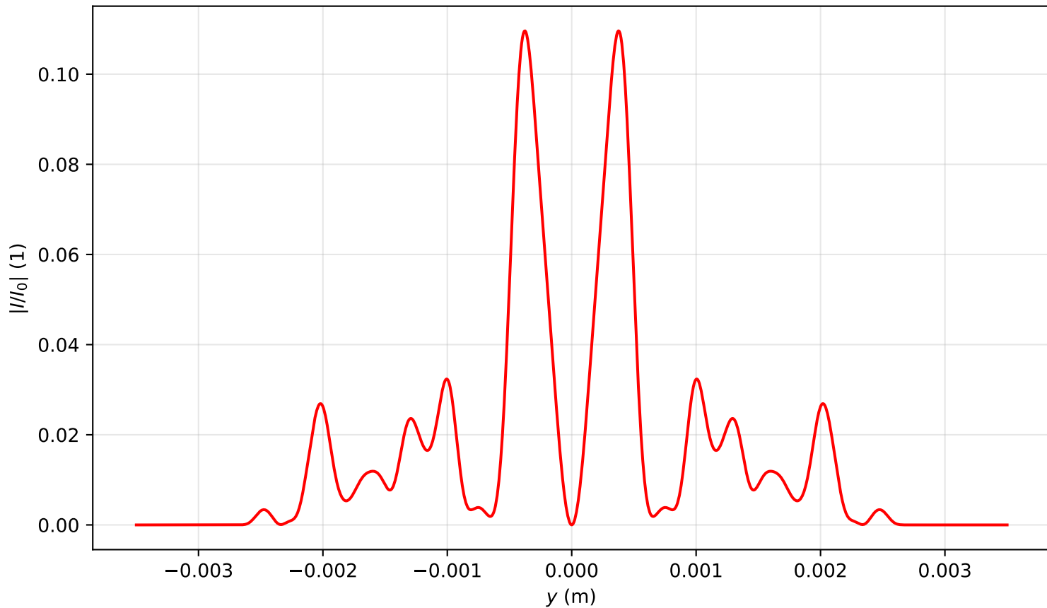
Intensity profile I(x=0, y, z=2.946)/I_0 , P_{in}=8.0P_{cr} , artificial time
